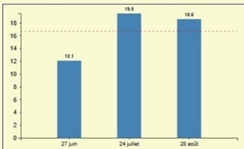
Concentration de chlorophylle a (µg/l)
